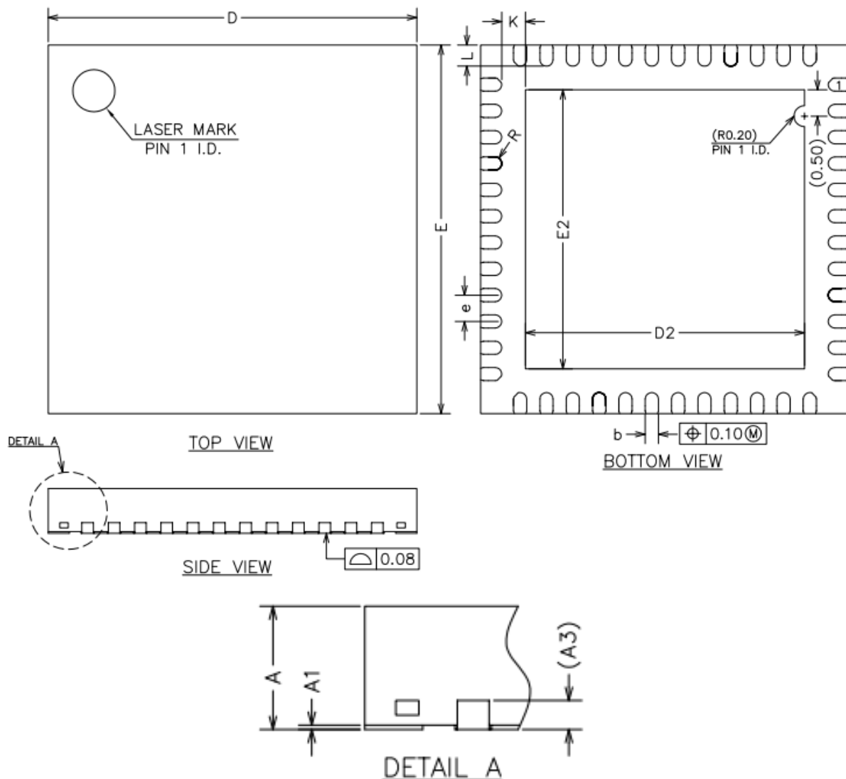
Figure 24 QFN48 Package Diagram
